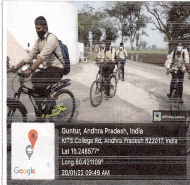
Bicycle
